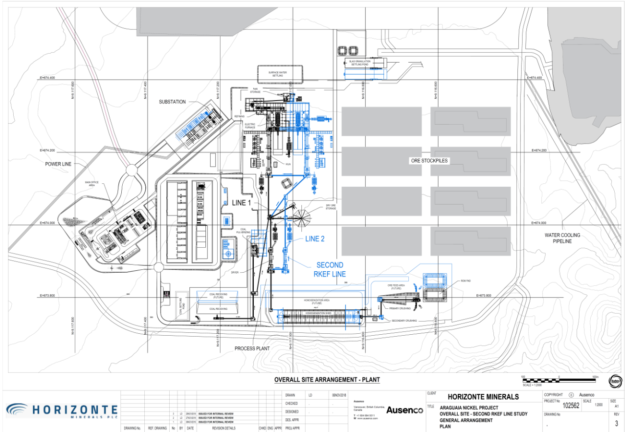
Figure 1 FS Plant layout with Stage 2 - Second line items shown in blue
